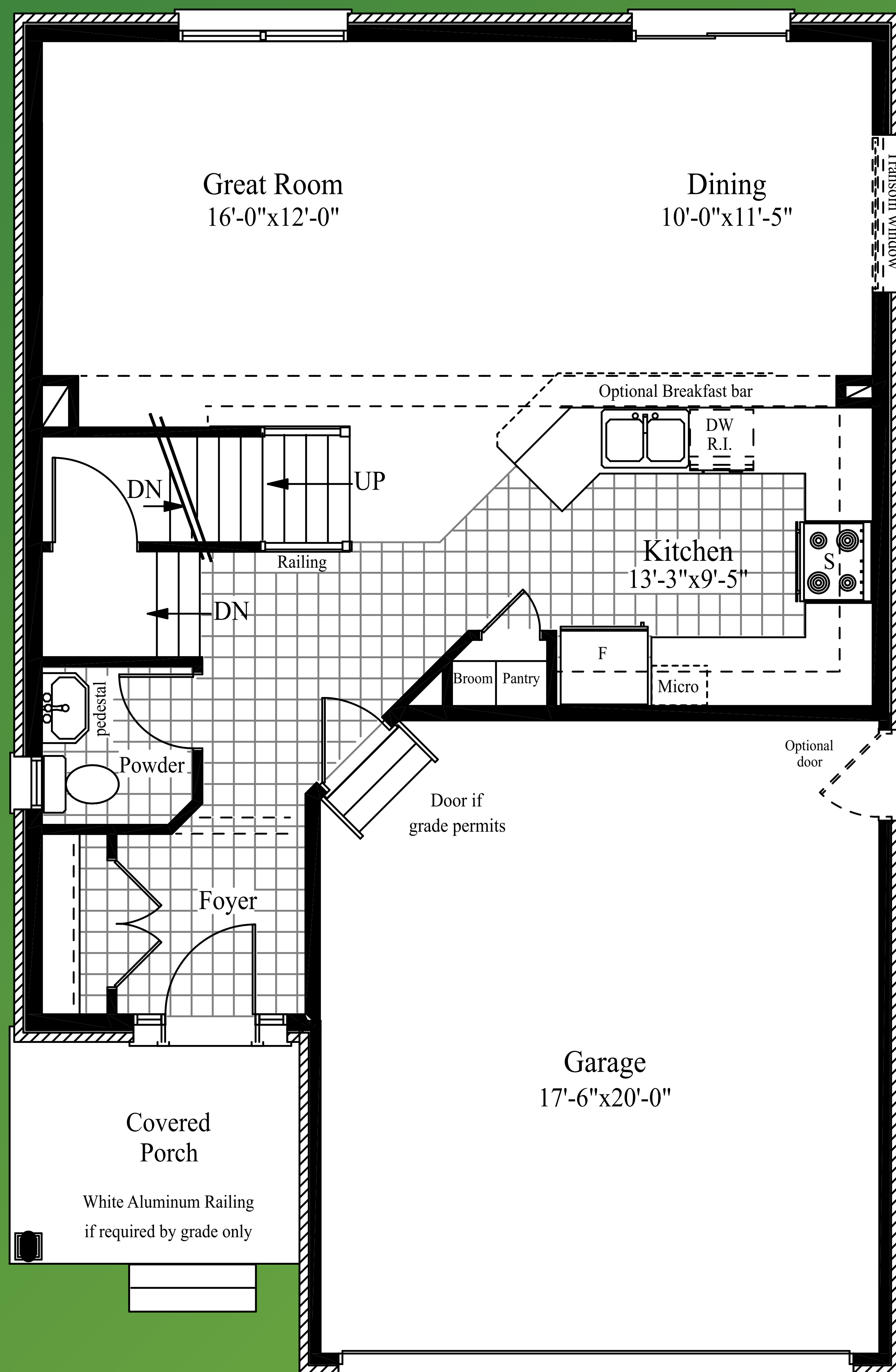
MAIN FLOOR
