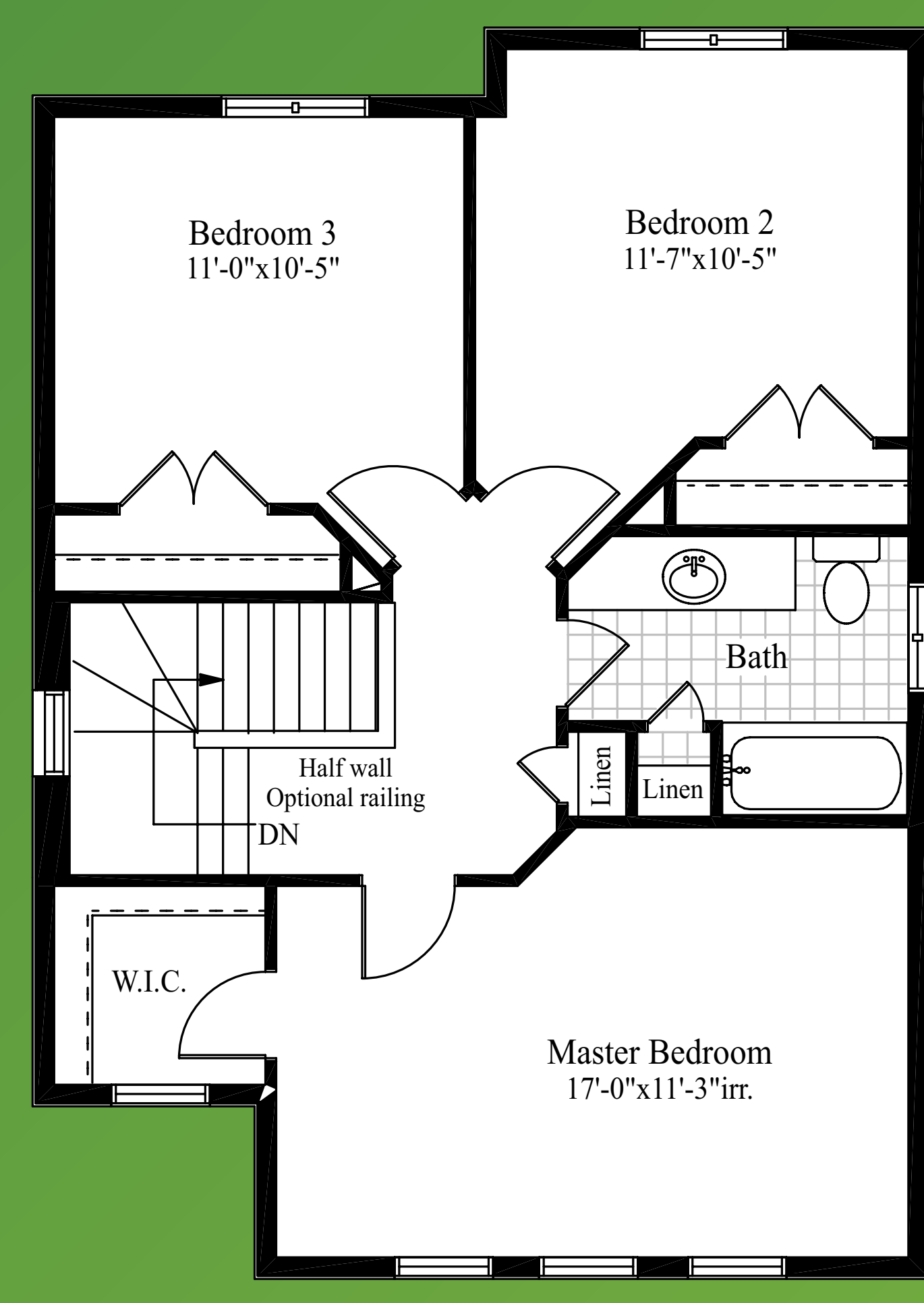
SECOND FLOOR
