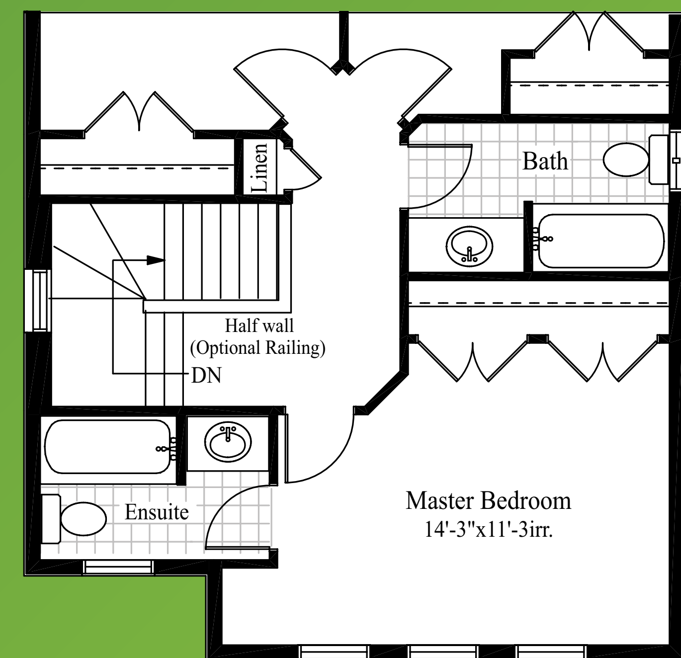
OPT. SECOND FLOOR: ENSUITE
