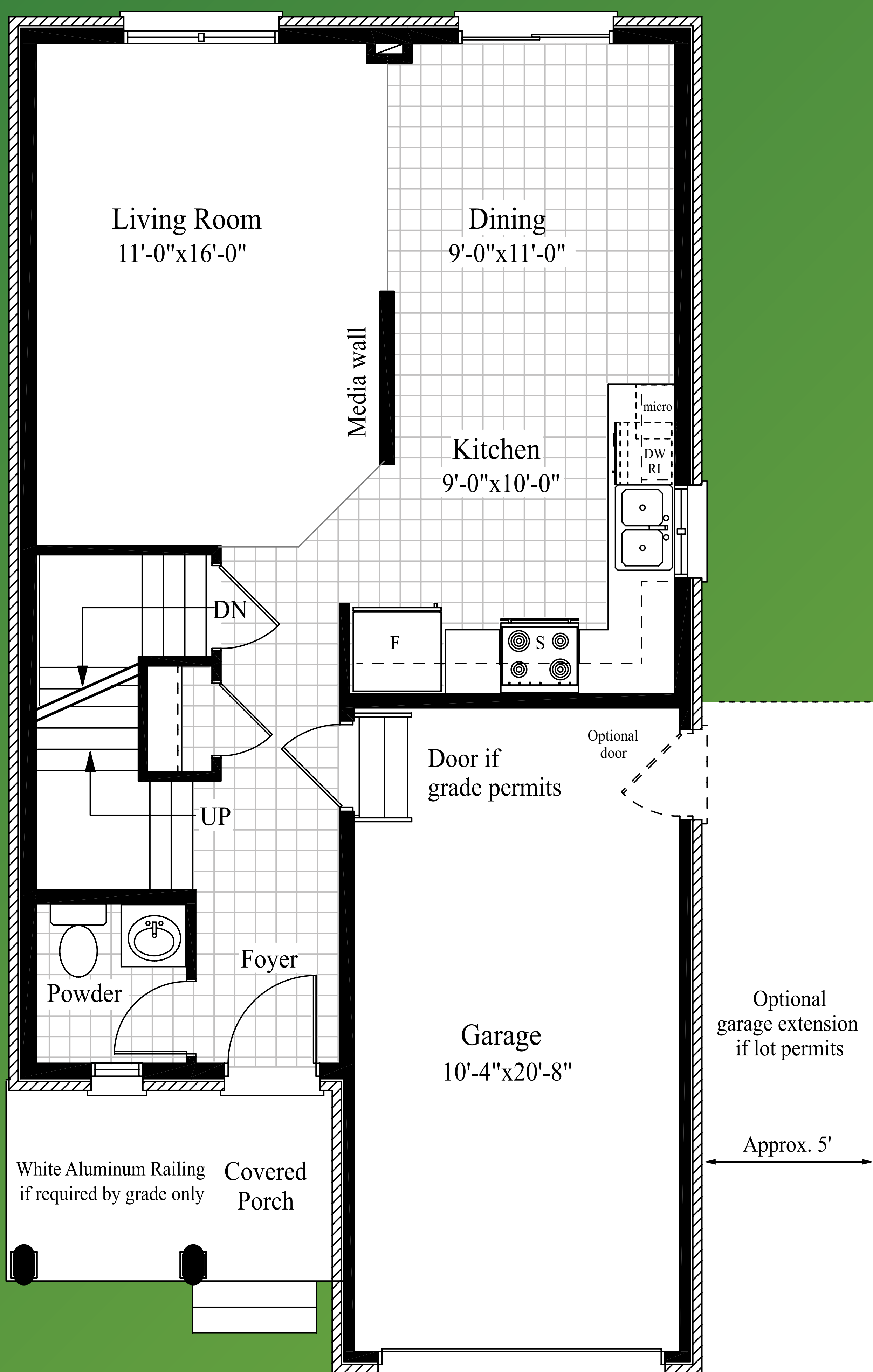
MAIN FLOOR
