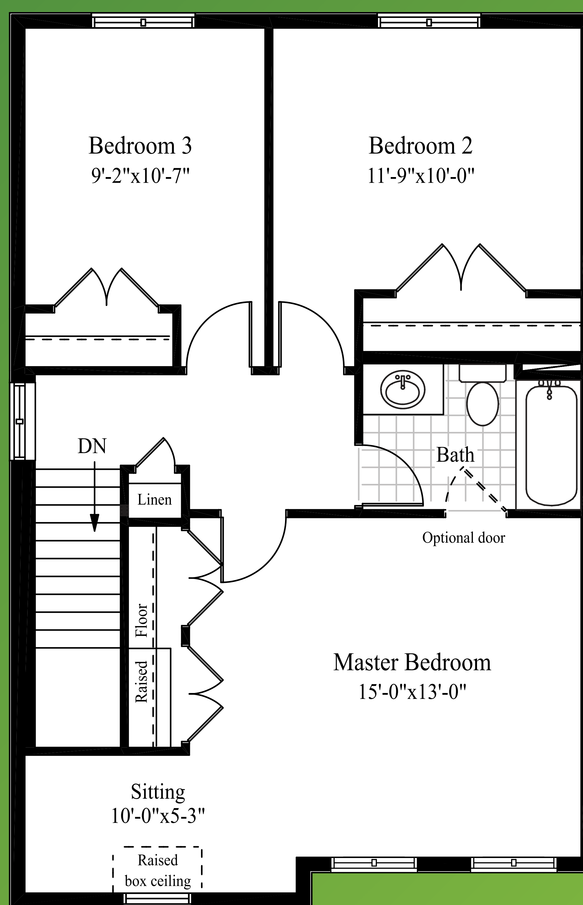
SECOND FLOOR
