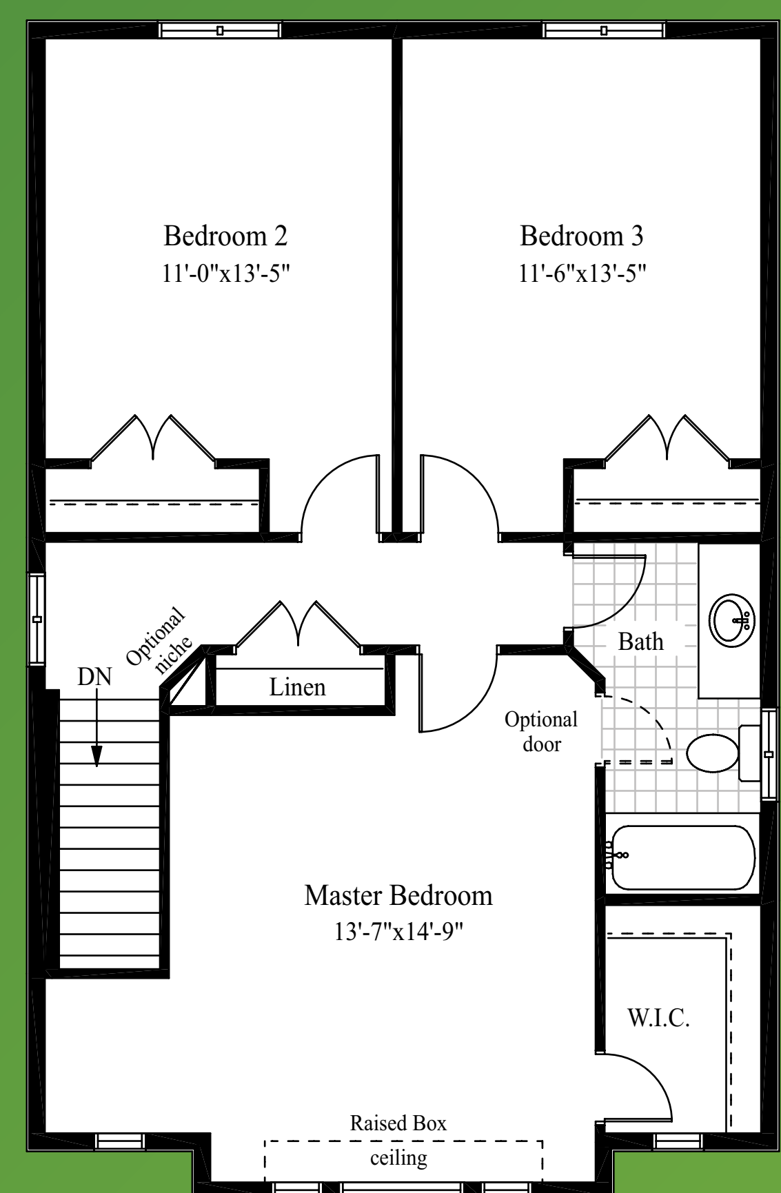
SECOND FLOOR
