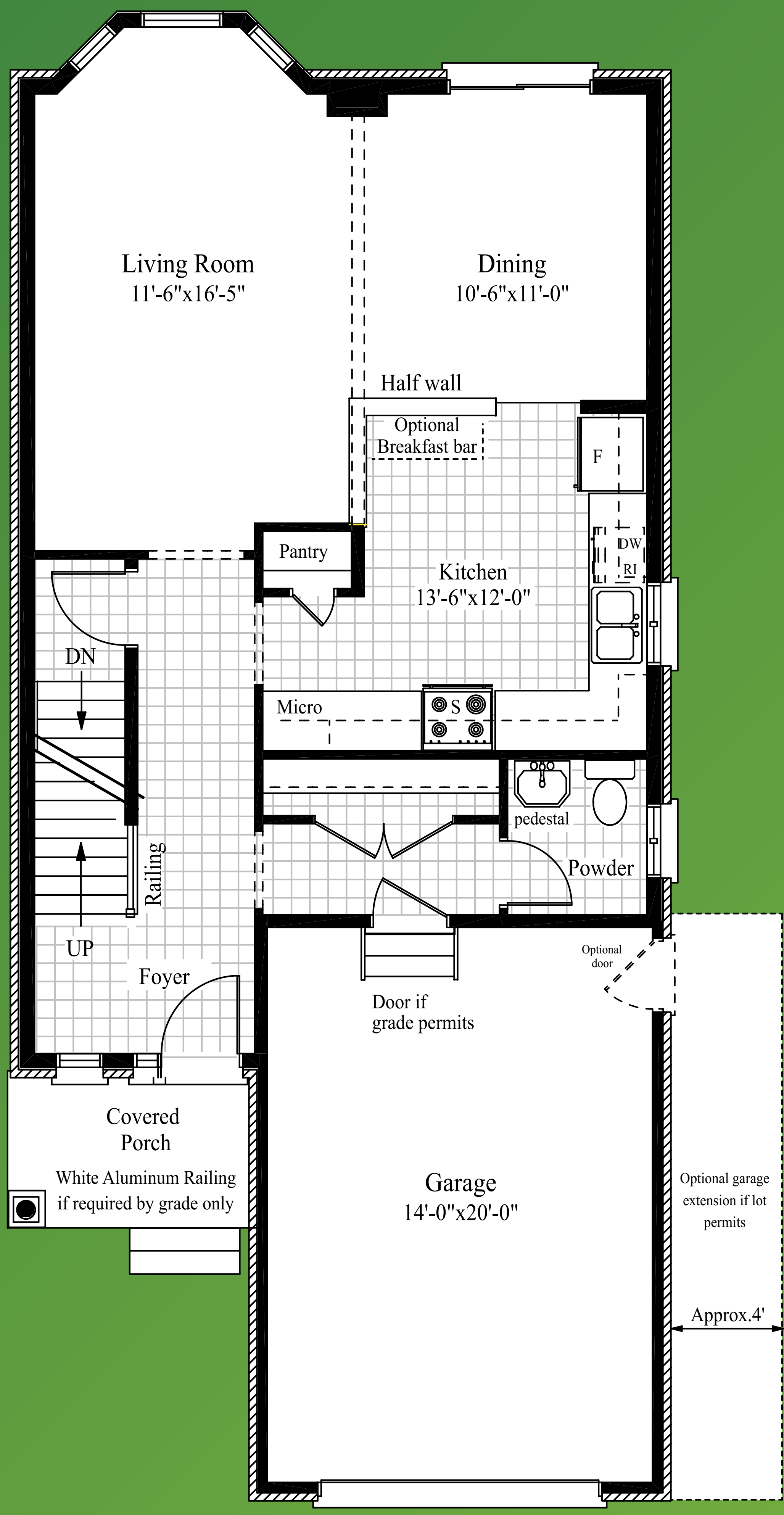
MAIN FLOOR
